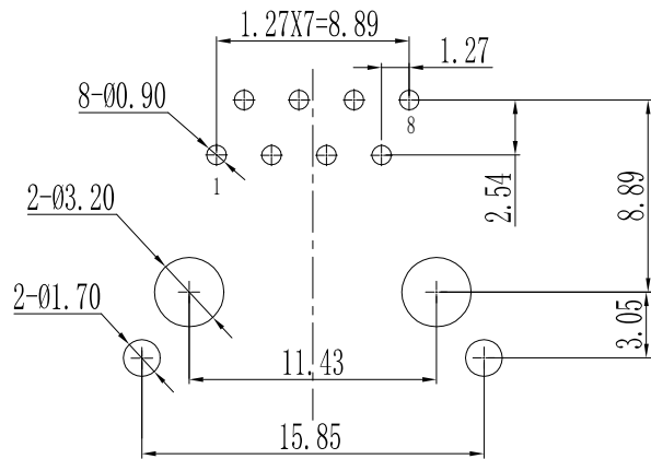
PCB LAYOUT ①
