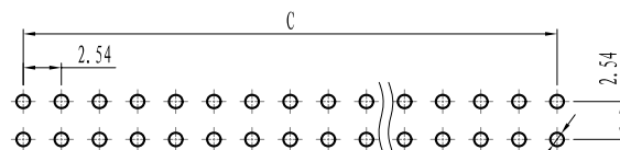
Referenced PCB LAYOUT tolerance: ± 0.05
