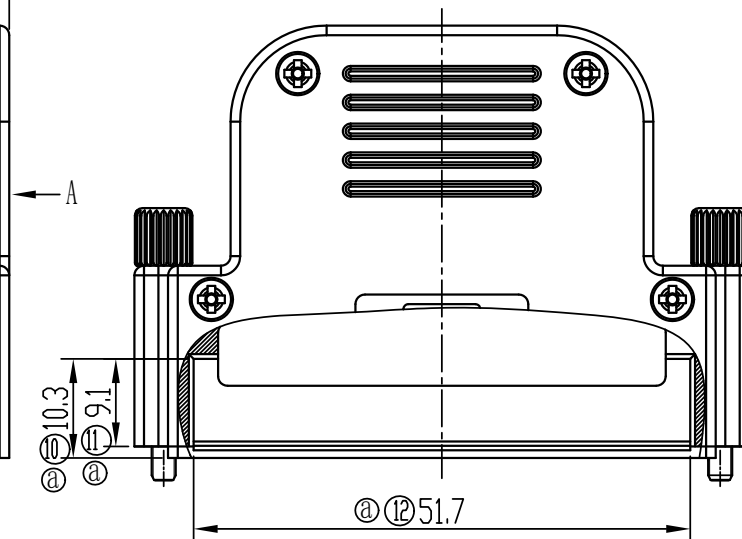
VIEW A
